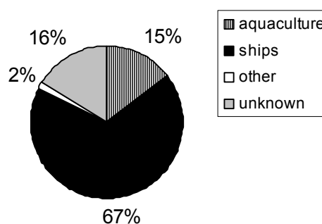
Figure 6. Introduction vectors of aquatic alien species in Belgian coastal waters
